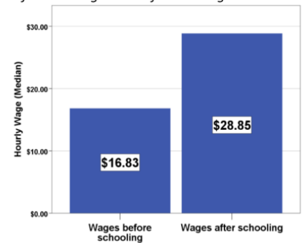
What were the hourly wages of the students before training versus after training?
